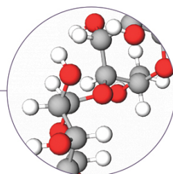
Pullulan
